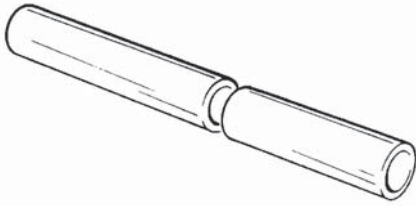
ø 48,4 mm x 3,35 mm wall HIGH TENSILE TUBE Mass 3,62 kg / Running meter
