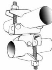
SWIVEL COUPLER 50 mm x 50 mm Mass 2,0 kg
