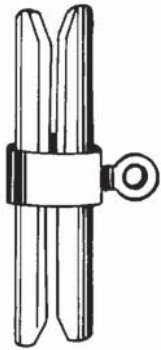
INTERNAL TUBE SPIGOT To fit ø 48,4 mm scaffold tube. Mass 0,9 kg
