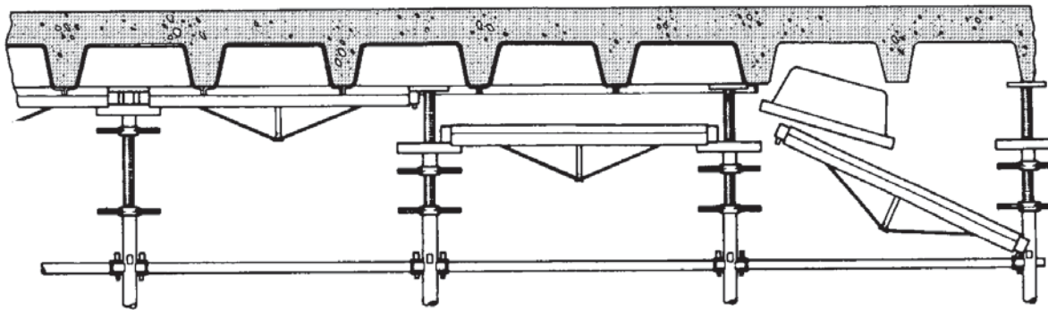
Stripping procedure of the Quick-Strip system
