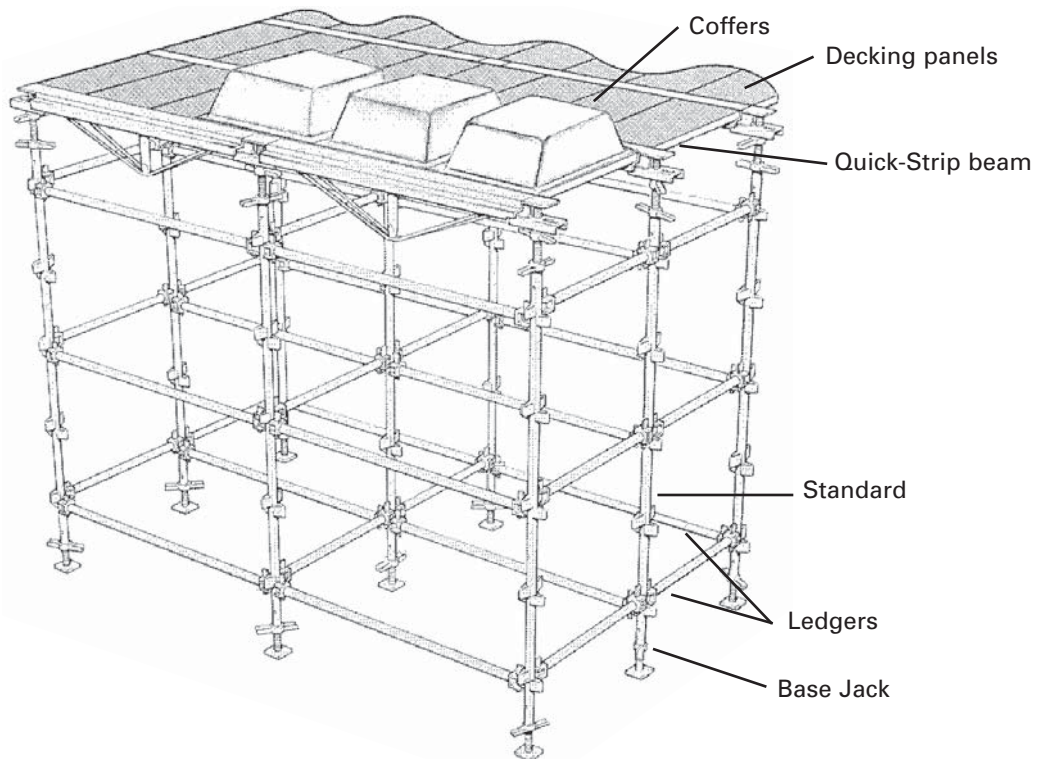
Wiehahn Quick-Strip System showing support versatility
